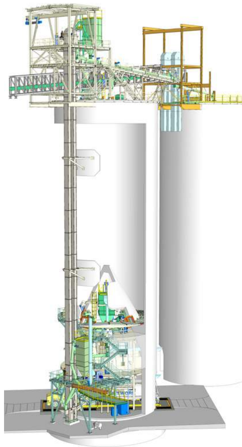
CEMENT SILO EXTRACTION
